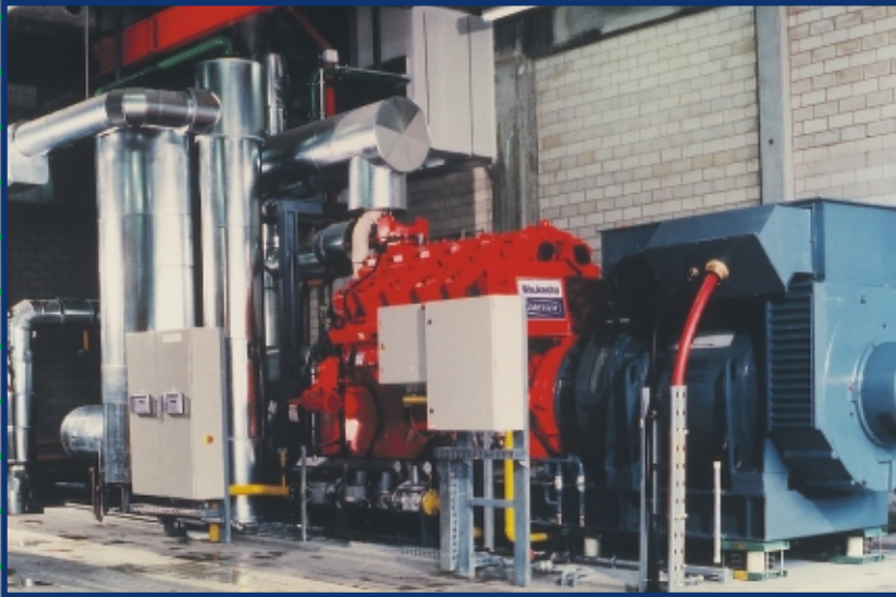
800-HP Natural Gas Engine/Generator
